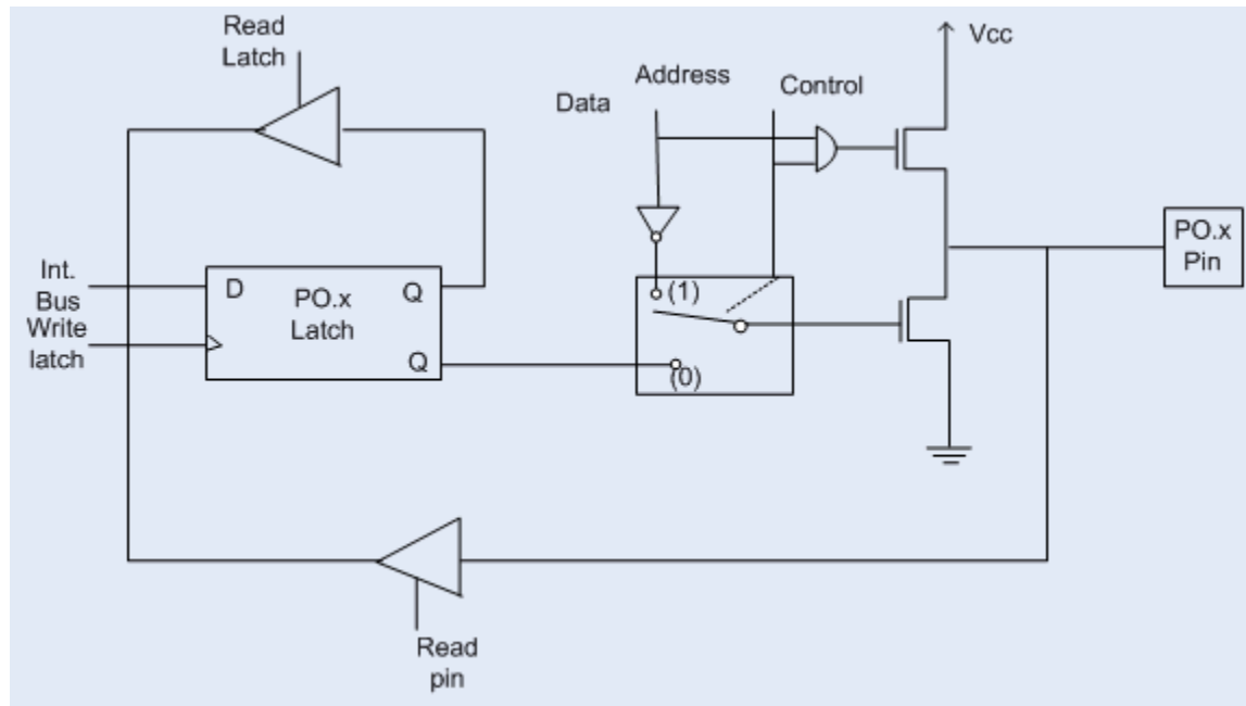
Fig 6.2: Port-0 Structure
