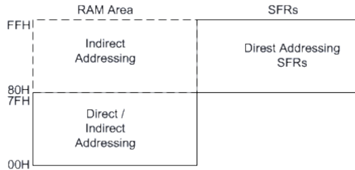
Fig 5.4 : Internal Data Memory Map
