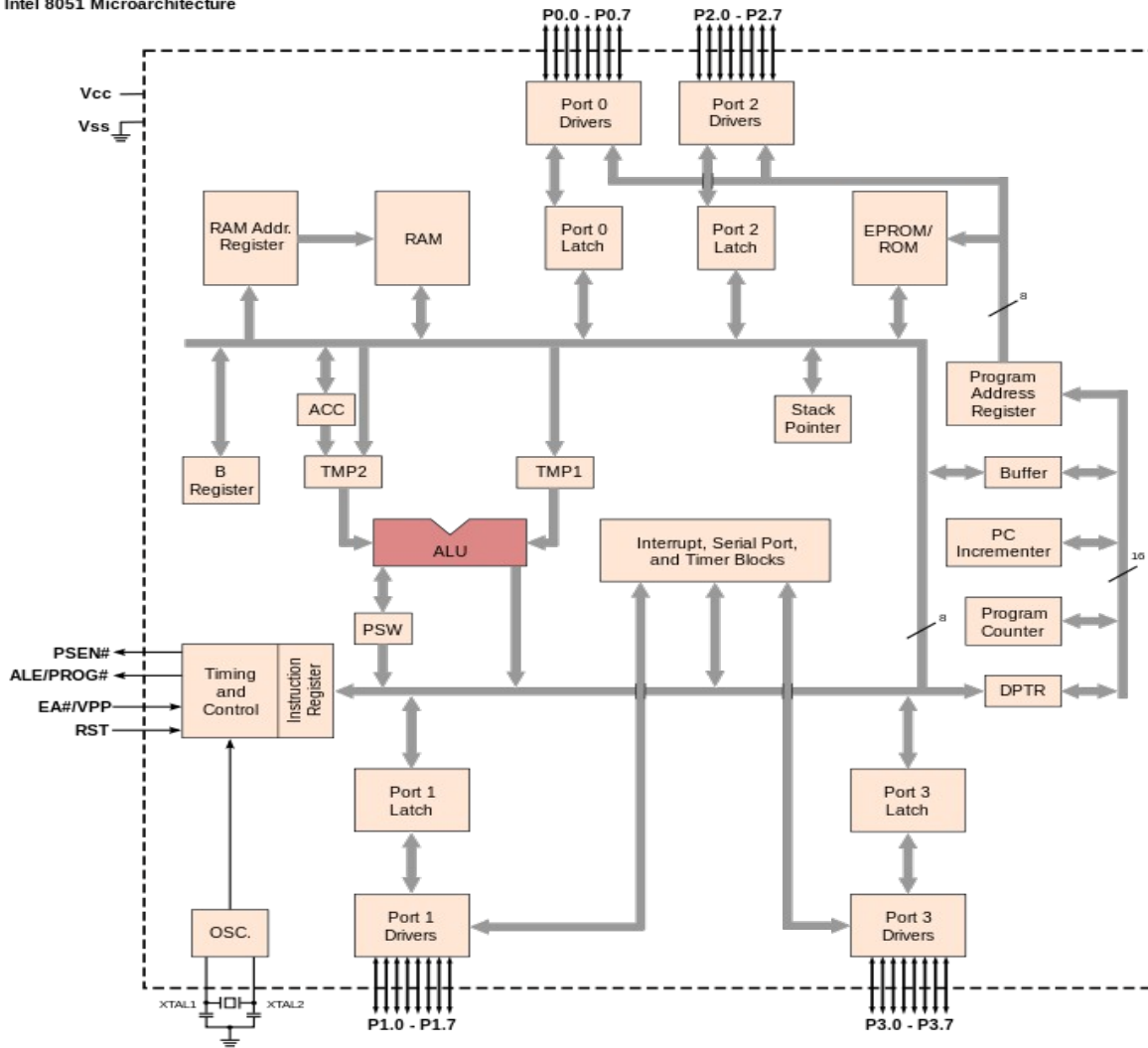
Intel 8051 Microarchitecture
