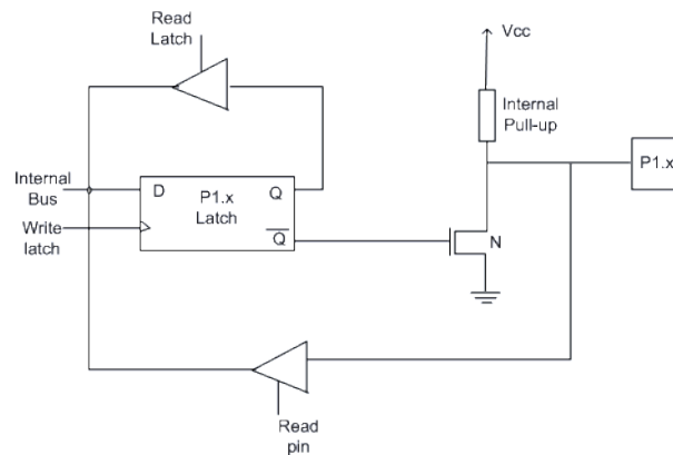
Fig 6.3 Port 1 Structure
